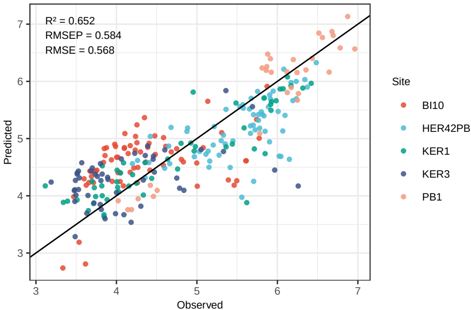
Mn PLS_kfold - Predicted vs Observed (log-space)
